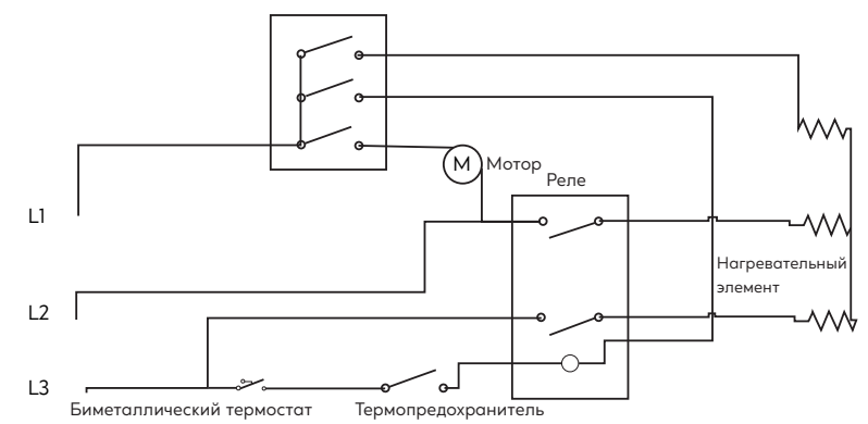
Модели TP-50S, TP-60S, TP-90S
